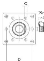
Pict. 5 _View of flange of in-parallel units and their fastenings
