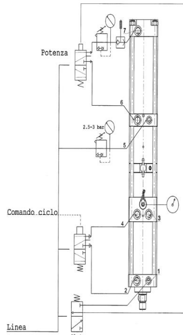
Picture 3 – pneumatic system_Version "E"
